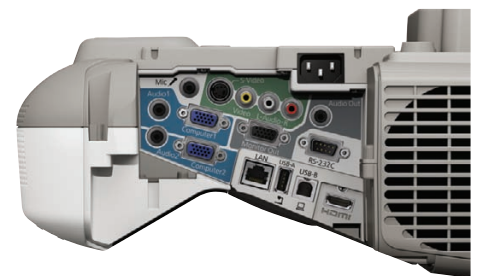
EB-485Wi interface
